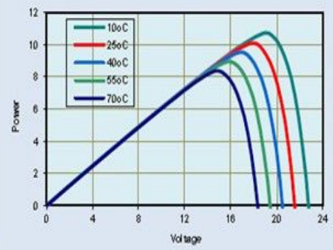
Power-Voltage Relationship, variable temperature
