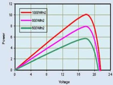
Power-Voltage Relationship, variable light intensity
