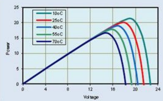
Power-Voltage Relationship, variable temperature
