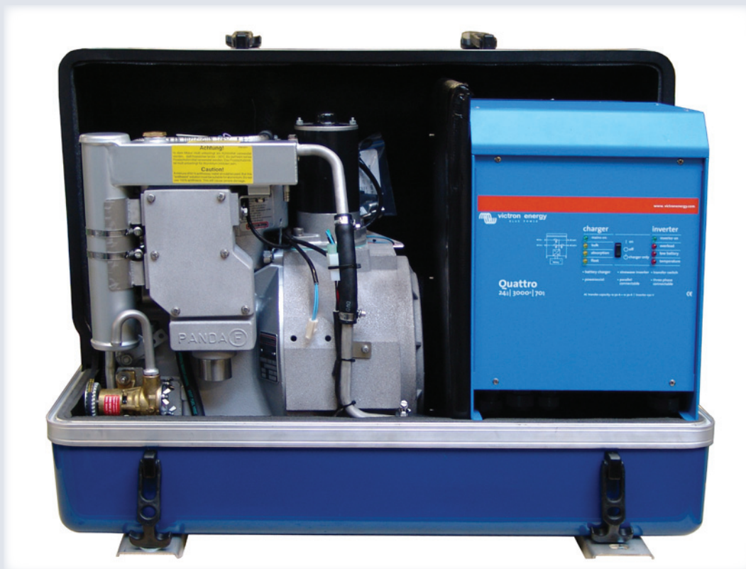
Photo 1: The HybridBox with a Victron Quattro 3kVA installed.
